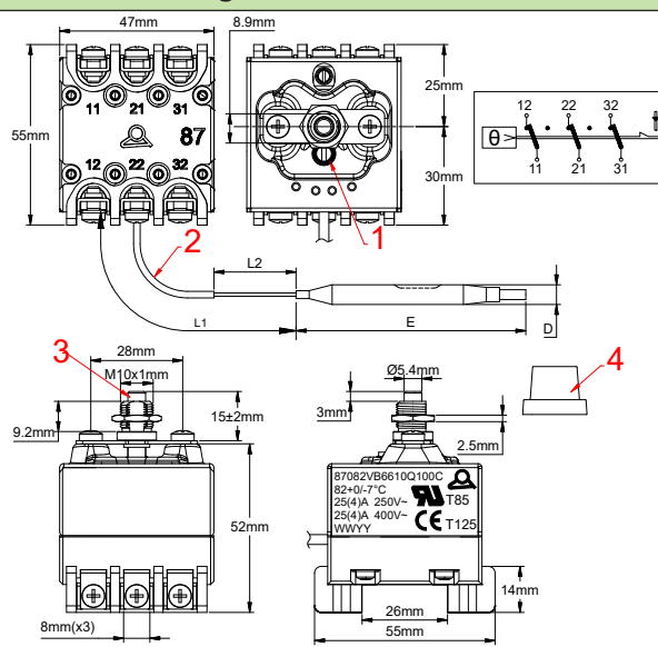
1. Sealing; 2. Sleeve; 3. Manual reset button; 4. Plastic cap(Black)
